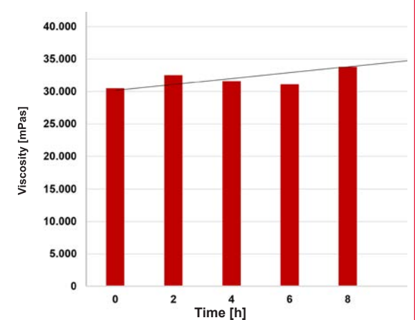
Viscosity curve | Jowatherm-Reaktant® (Test temperature 135 °C)
